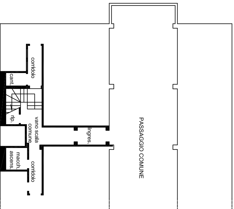
PIANO INTERRATO 17-513-60
